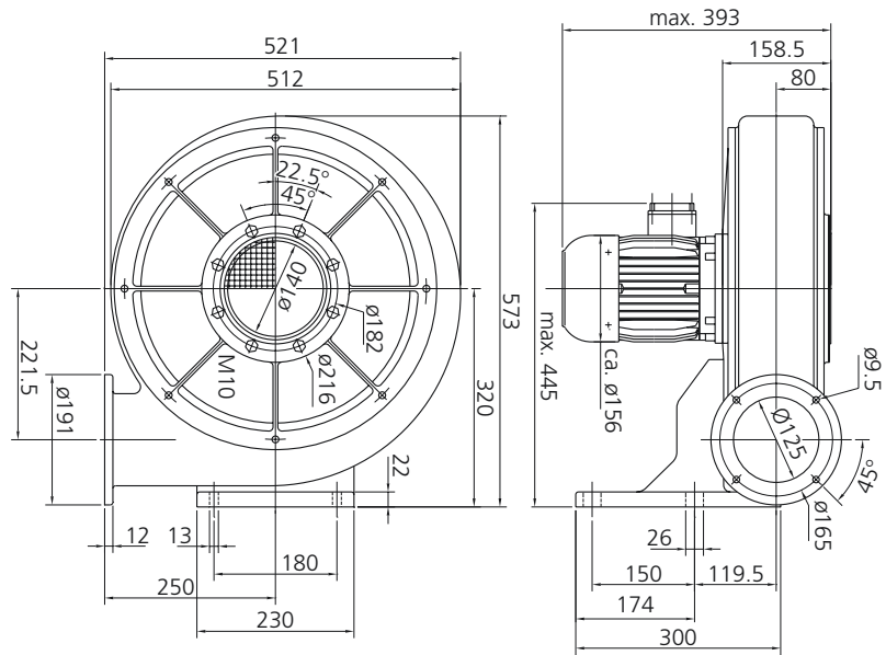
Maße in mm – unverbindlich Dimensions in mm – subject to modifications
